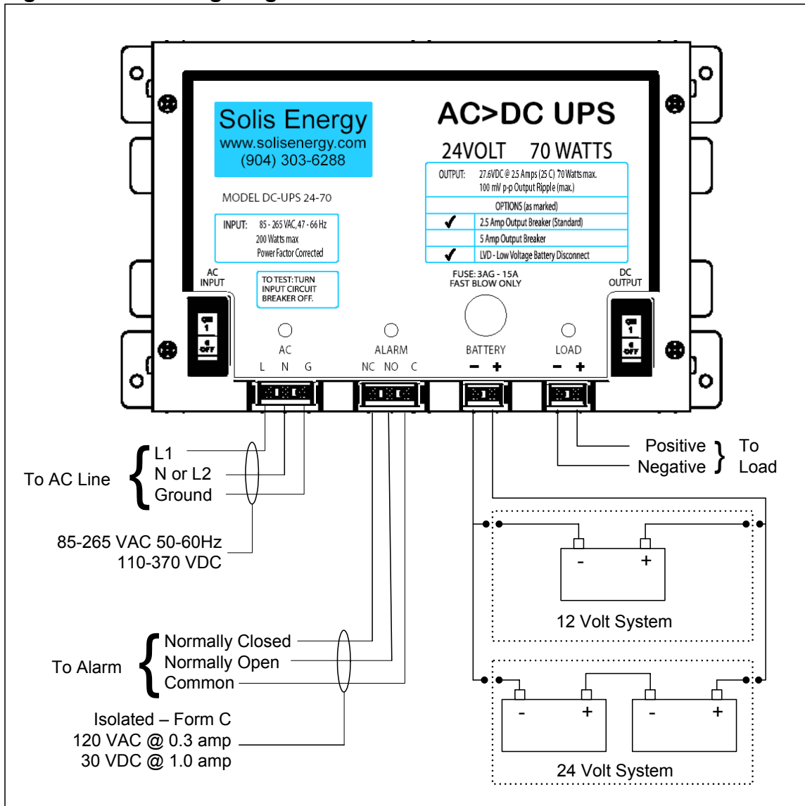
Figure 7.3.1 – Wiring Diagram
