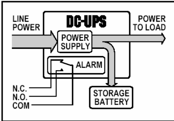
Figure 4.1.1 – Operation in LINE-UP Mode.
