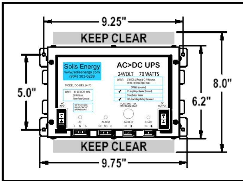
Figure 7.2.1 – Flat Panel Mounting
