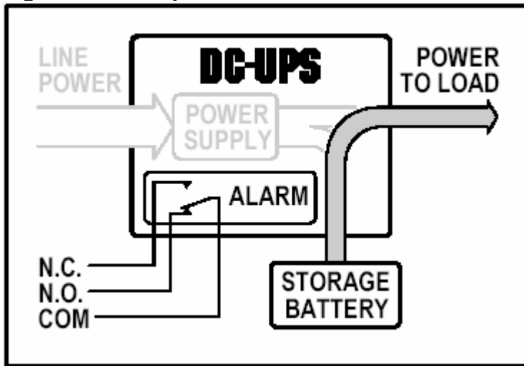
Figure 4.2.1 – Operation in LINE-DOWN Mode.
