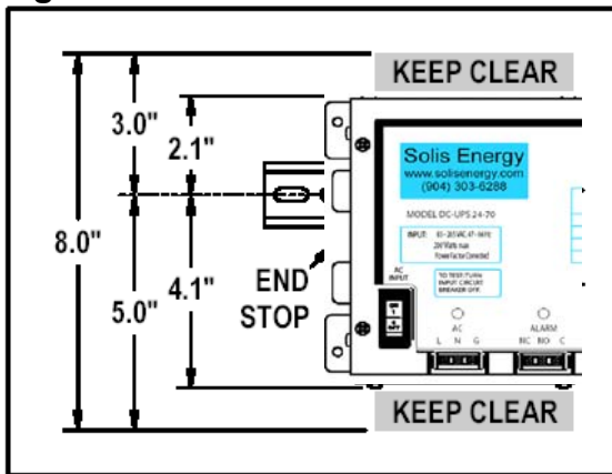
Figure 7.2.3 – Low Position DIN Mounting.
