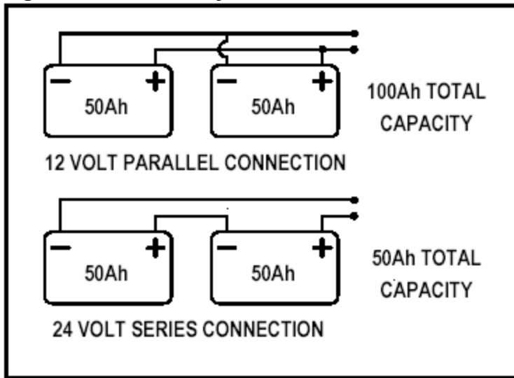
Figure 6.4.2 – Battery Banks
