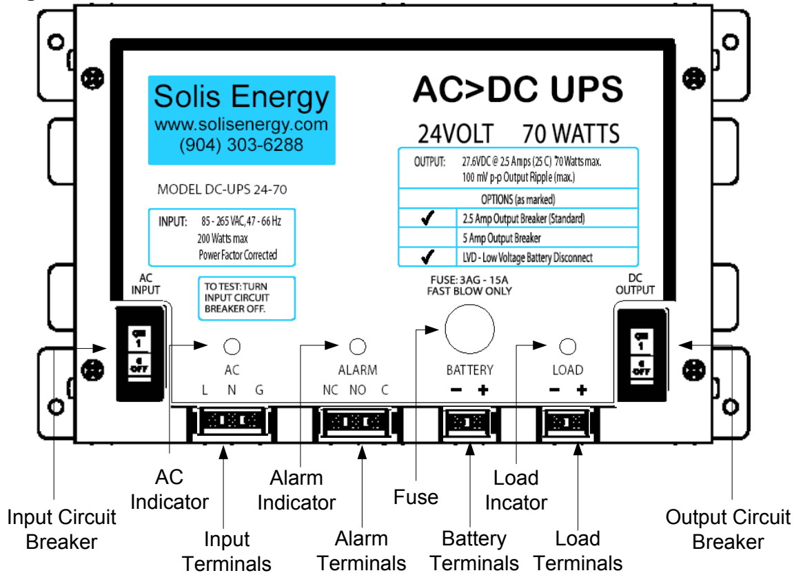
Figure 8.0.1 – General View
