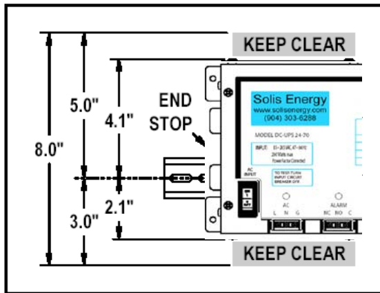
Figure 7.2.2 – High Position DIN Mounting.
